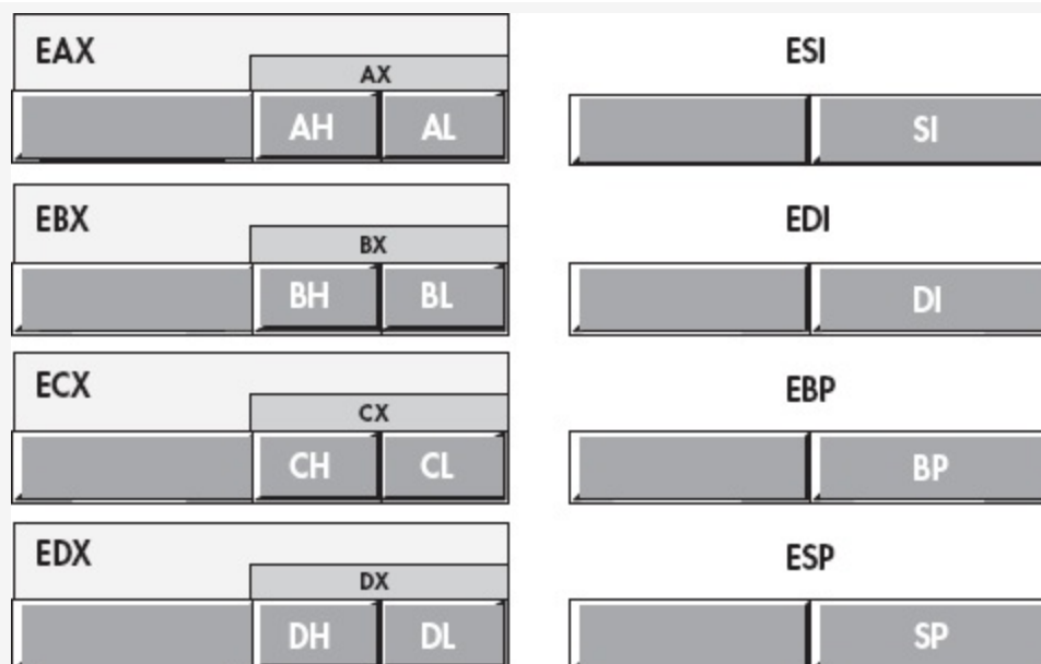
Figure 1-5. 80x86 (Intel CPU) general-purpose registers
