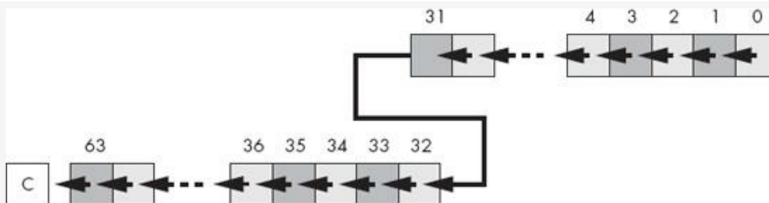
Figure 8-5. 64-bit shift-left operation
