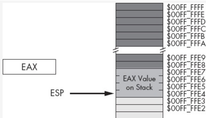
Figure 3-11. Memory before a pop( eax ); operation
