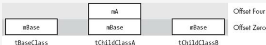
Figure 12-8. Virtual method tables for inherited classes
