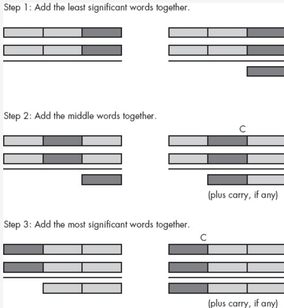
Figure 8-1. Adding two 96-bit objects together
