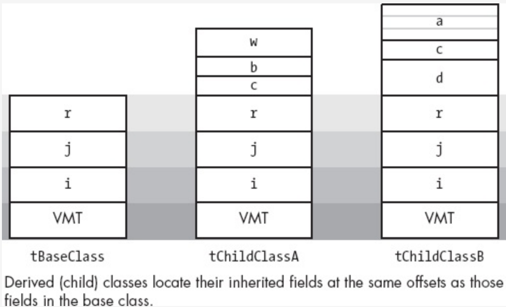
Figure 12-6. Layout of base and child class objects in memory
