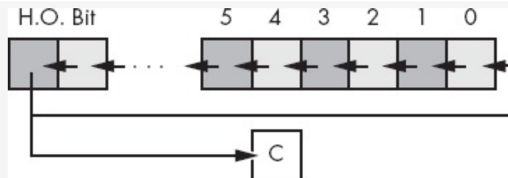
Figure 2-15. rol( 1, dest ) operation
