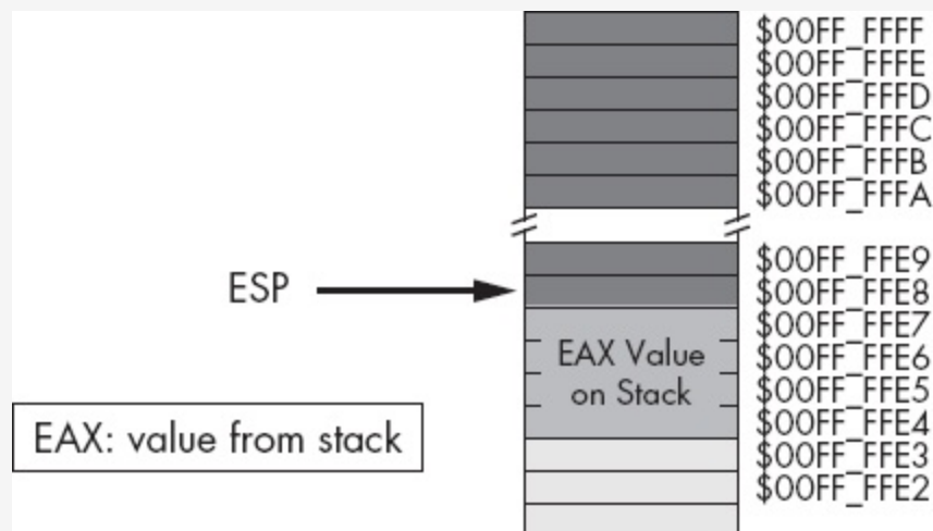
Figure 3-12. Memory after the pop( eax ); instruction
