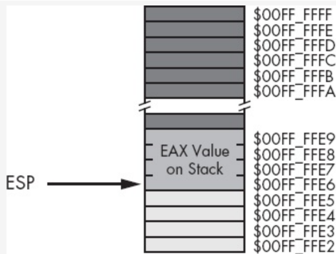
Figure 3-13. Stack after pushing EAX
