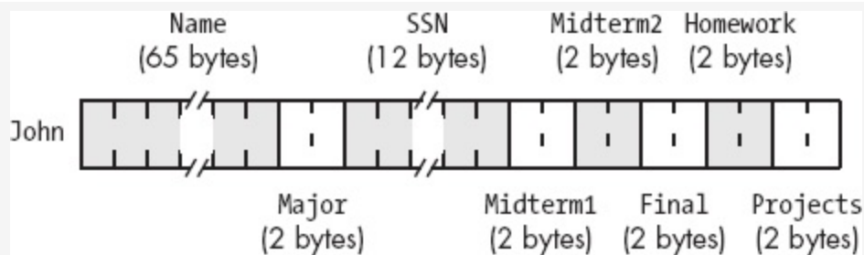
Figure 4-10. Student data structure storage in memory
