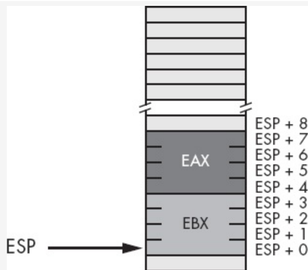
Figure 3-19. Stack after pushing EAX and EBX
