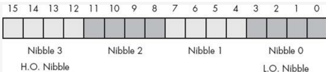
Figure 2-5. Nibbles in a word
