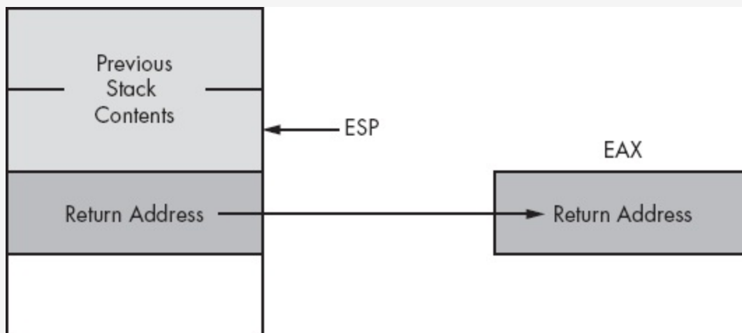
Figure 5-2. Stack contents before ret in messedUpToo
