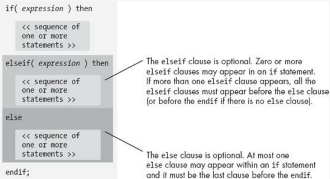
Figure 1-10. HLA if statement syntax
