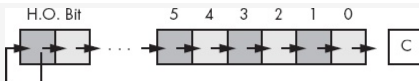
Figure 2-13. sar( 1, dest ) operation
