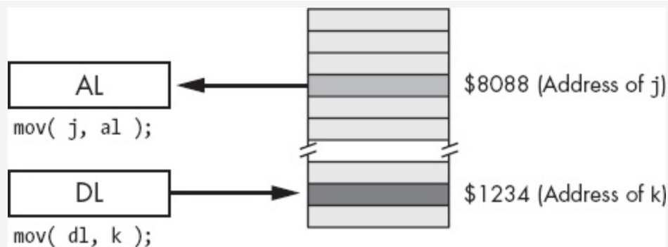
Figure 3-1. Displacement-only (direct) addressing mode
