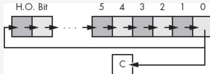
Figure 2-16. ror( 1, dest ) operation
