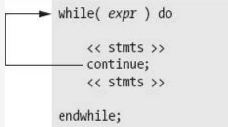
Figure 7-3. continue destination and the while loop
