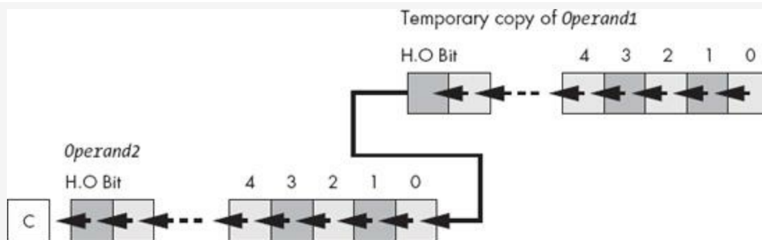
Figure 8-6. shld operation
