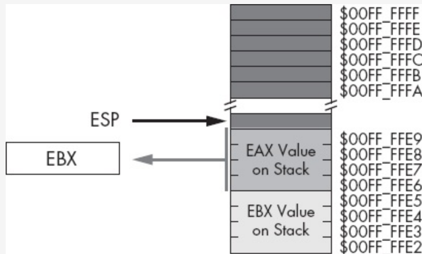
Figure 3-16. Stack after popping EBX
