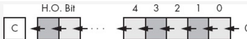
Figure 2-9. Shift-left operation
