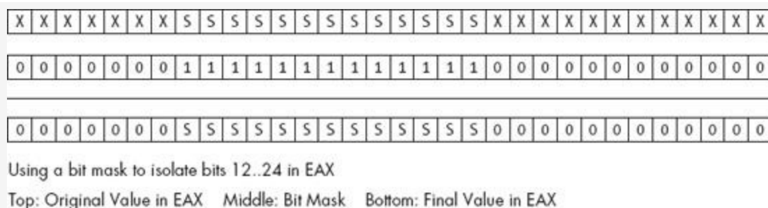
Figure 10-1. Isolating a bit string using the and instruction
