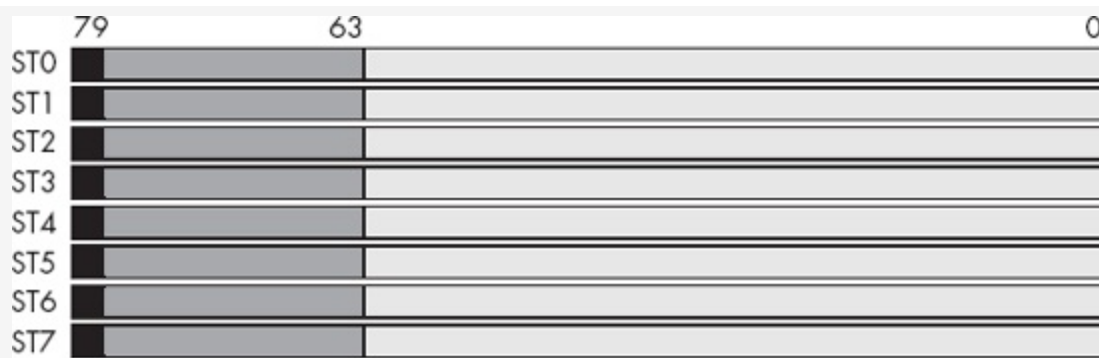
Figure 6-1. FPU floating-point register stack
