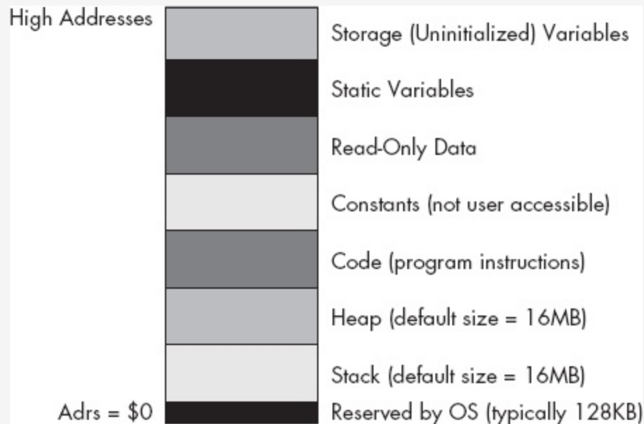
Figure 3-7. HLA typical runtime memory organization
