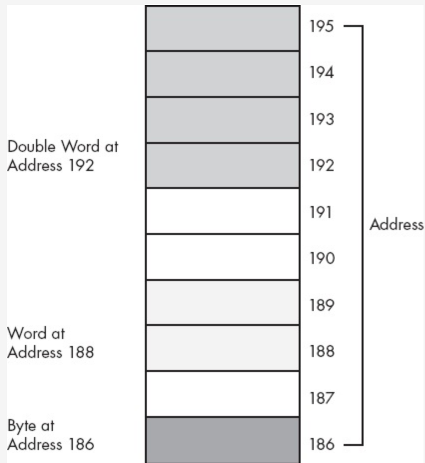
Figure 1-9. Byte, word, and double-word storage in memory
