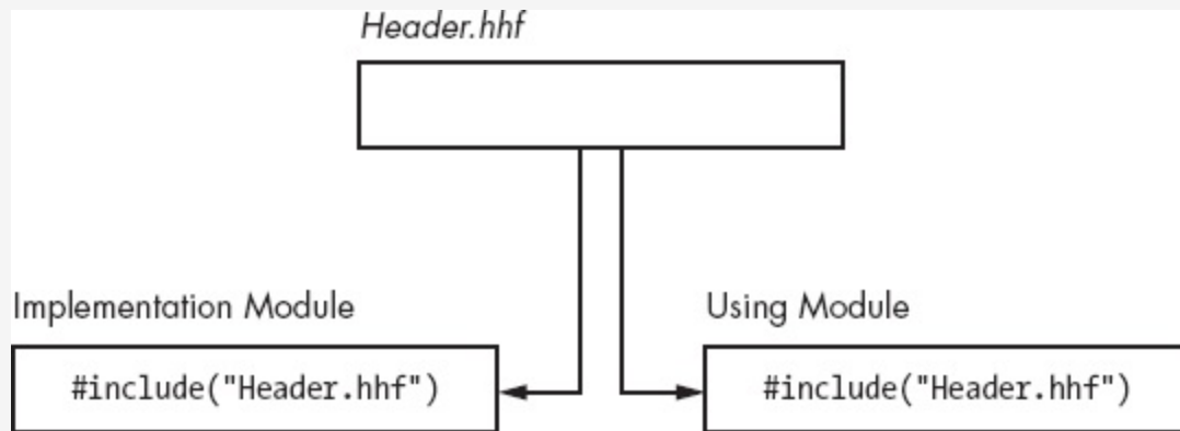
Figure 5-10. Using header files in HLA programs
