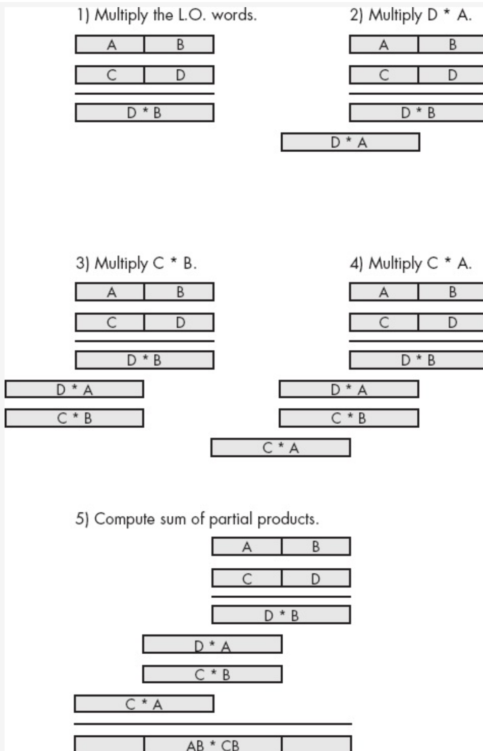
Figure 8-2. Extended-precision multiplication
