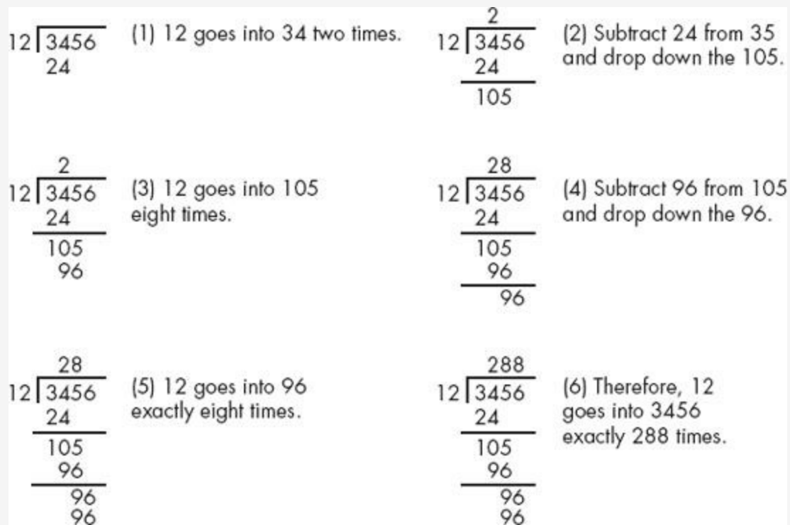
Figure 8-3. Manual digit-by-digit division operation
