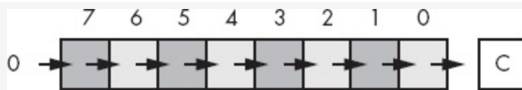
Figure 2-10. Shift-right operation
