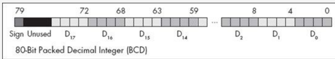
Figure 6-6. FPU packed decimal format
