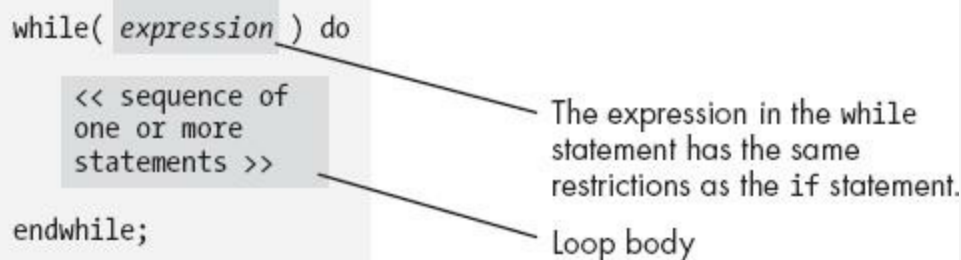
Figure 1-11. HLA while statement syntax
