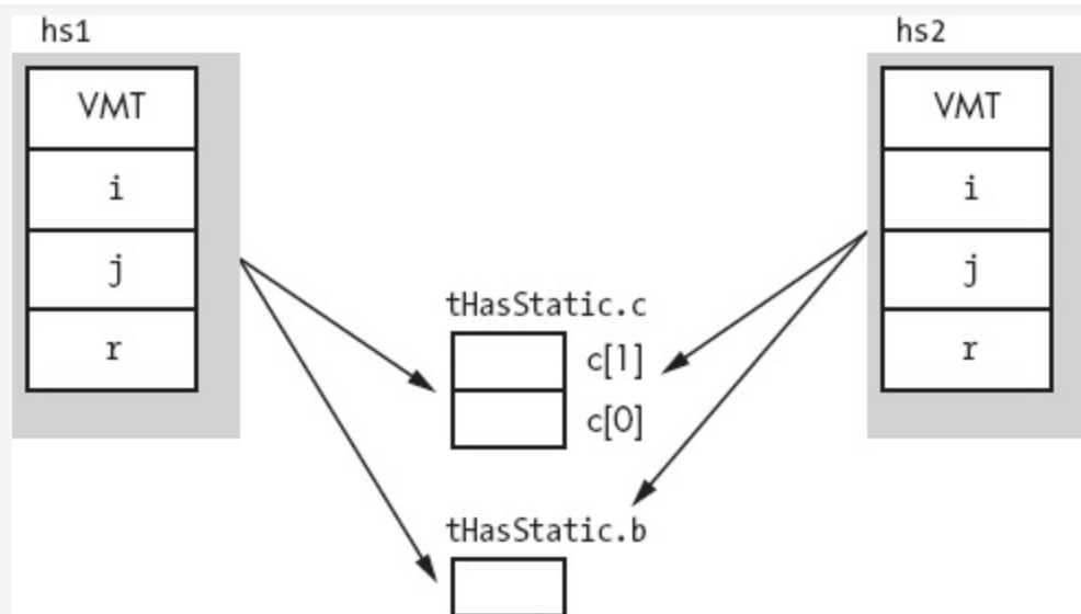
Figure 12-3. Object allocation with static data fields
