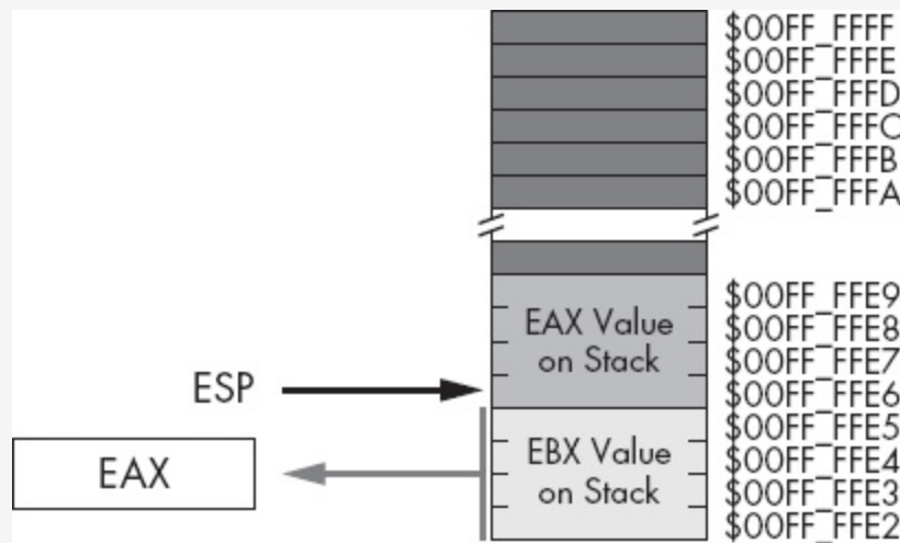
Figure 3-15. Stack after popping EAX
