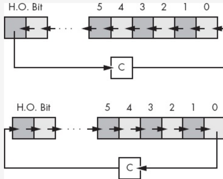
Figure 2-17. rcl( 1, dest ) and rcr( 1, dest ) operations
