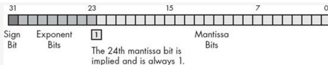
Figure 2-22. Single-precision (32-bit) floating-point format
