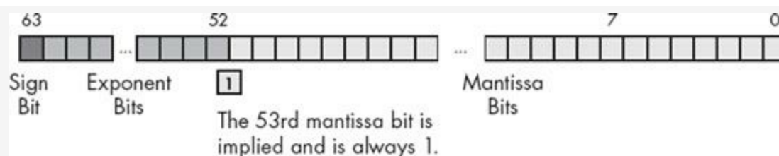
Figure 2-23. 64-bit double-precision floating-point format
