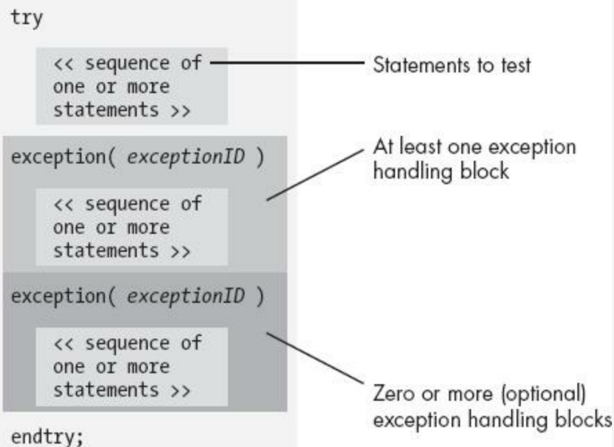
Figure 1-15. HLA try..exception..endtry statement syntax
