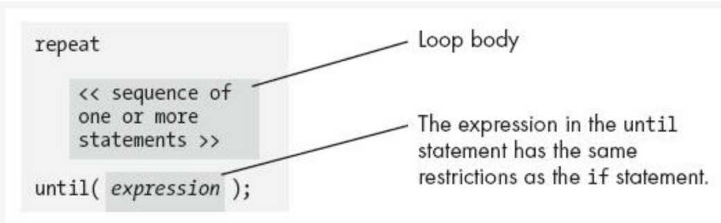
Figure 1-12. HLA repeat..until statement syntax
