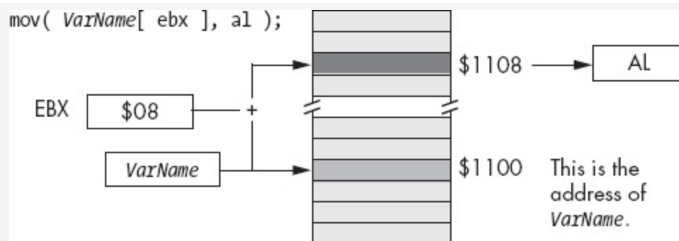
Figure 3-3. Indexed addressing mode
