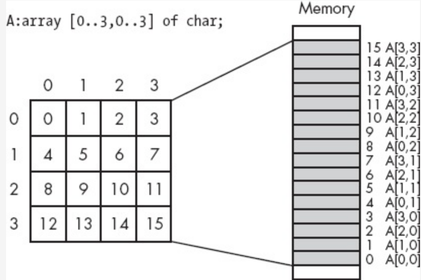
Figure 4-9. Column-major array element ordering
