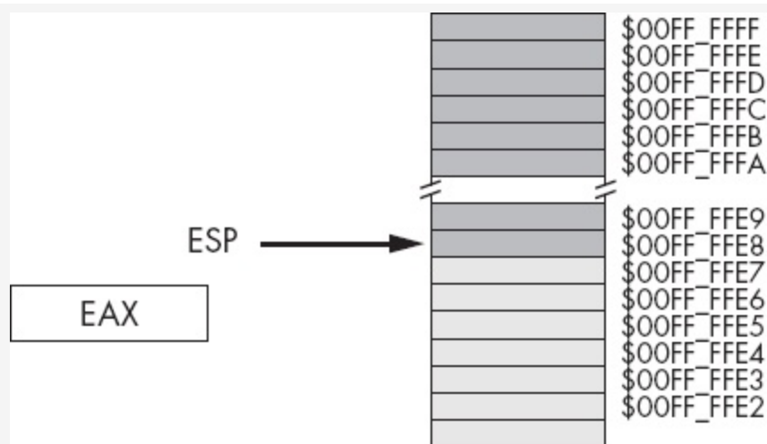
Figure 3-9. Stack segment before the push( eax ); operation
