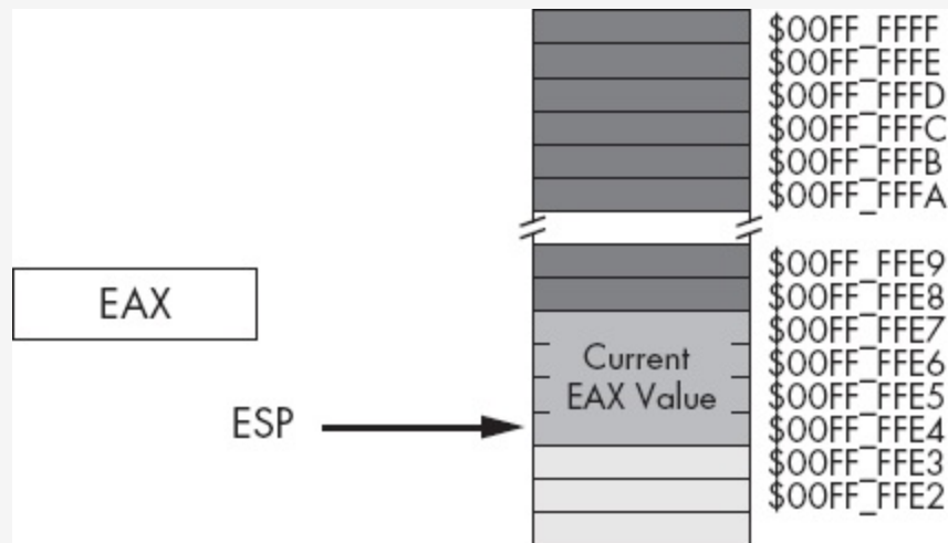
Figure 3-10. Stack segment after the push( eax ); operation
