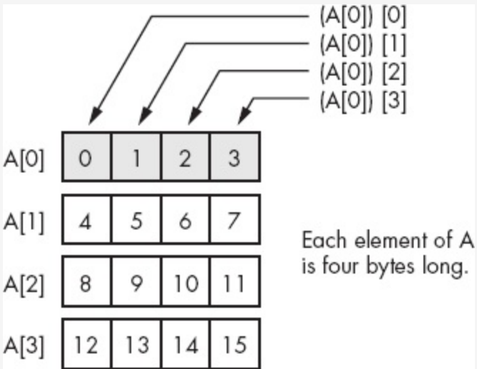
Figure 4-8. Viewing a 4x4 array as an array of arrays
