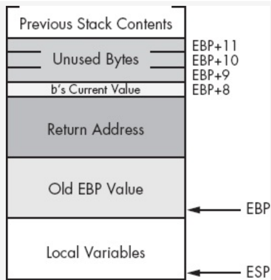
Figure 5-9. OneByteParm activation record
