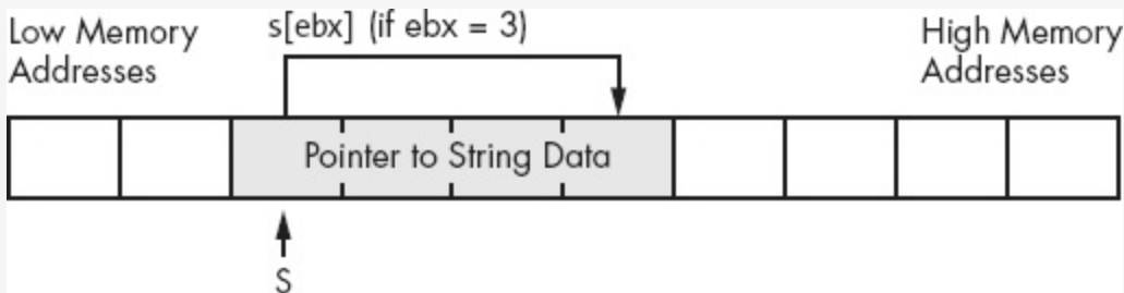
Figure 4-1. Incorrectly indexing off a string variable
