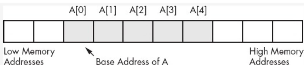
Figure 4-4. Array layout in memory
