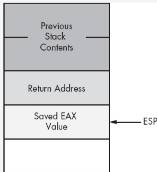
Figure 5-1. Stack contents before ret in MessedUp procedure
