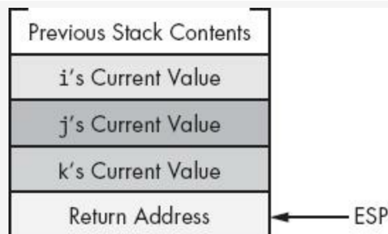
Figure 5-7. Stack layout upon entry into CallProc
