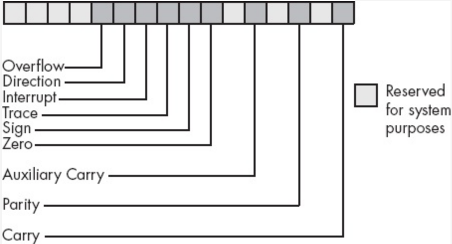
Figure 2-20. EFLAGS register as packed boolean data
