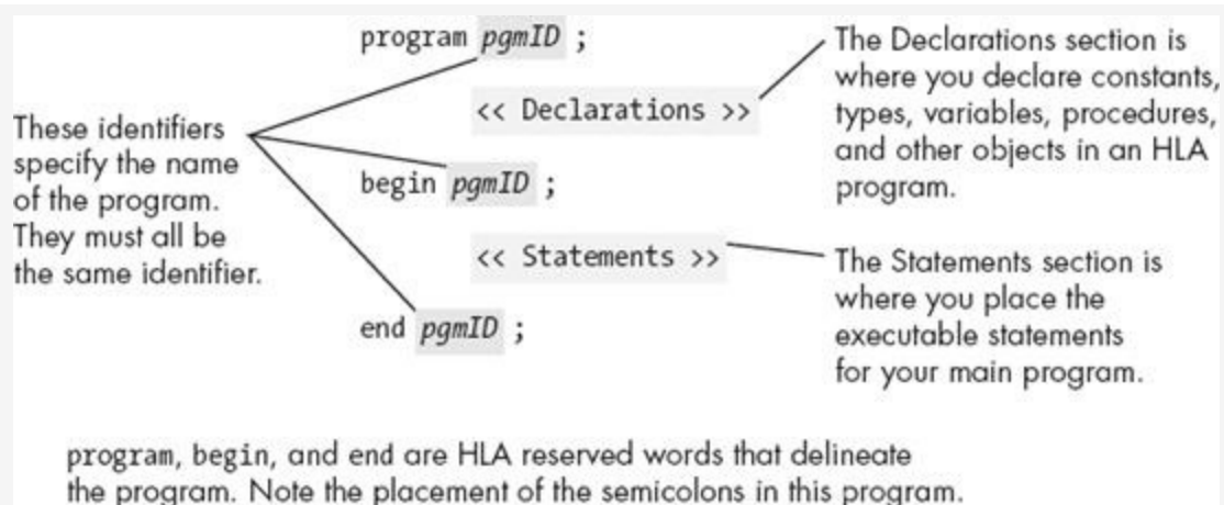
Figure 1-1. Basic HLA program
