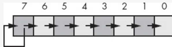
Figure 2-12. Arithmetic shift-right operation
