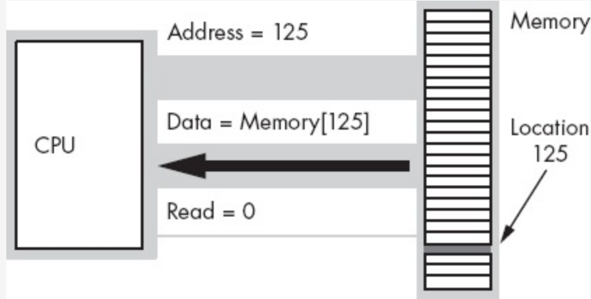
Figure 1-8. Memory read operation
