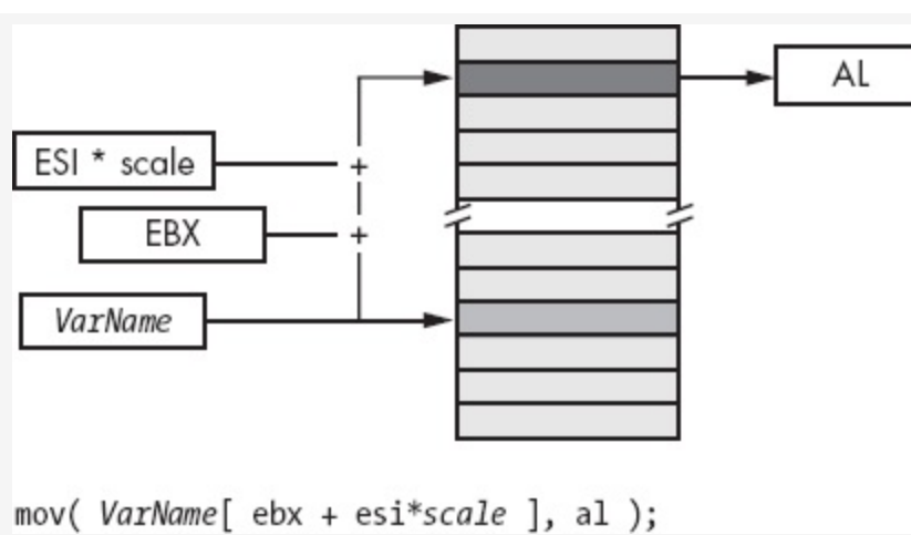
Figure 3-6. Scaled-indexed addressing mode
