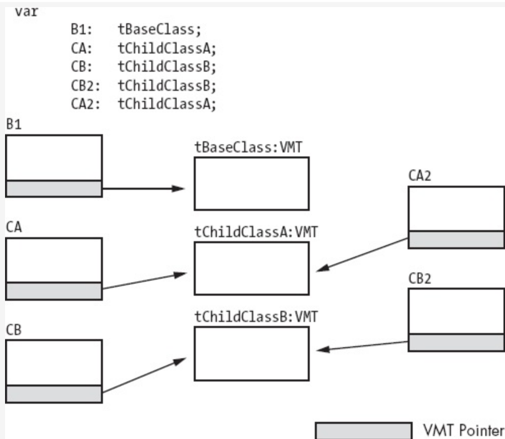
Figure 12-7. Virtual method table references from objects
