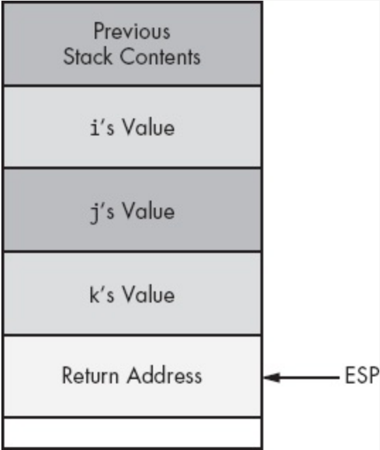
Figure 5-3. Stack organization immediately upon entry into ARDemo
