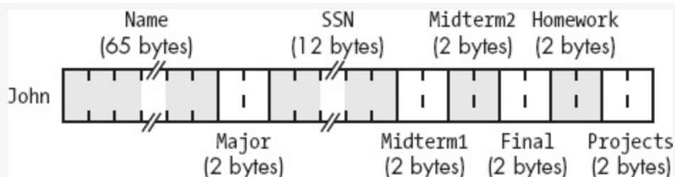
Figure 12-1. student record implementation in memory
