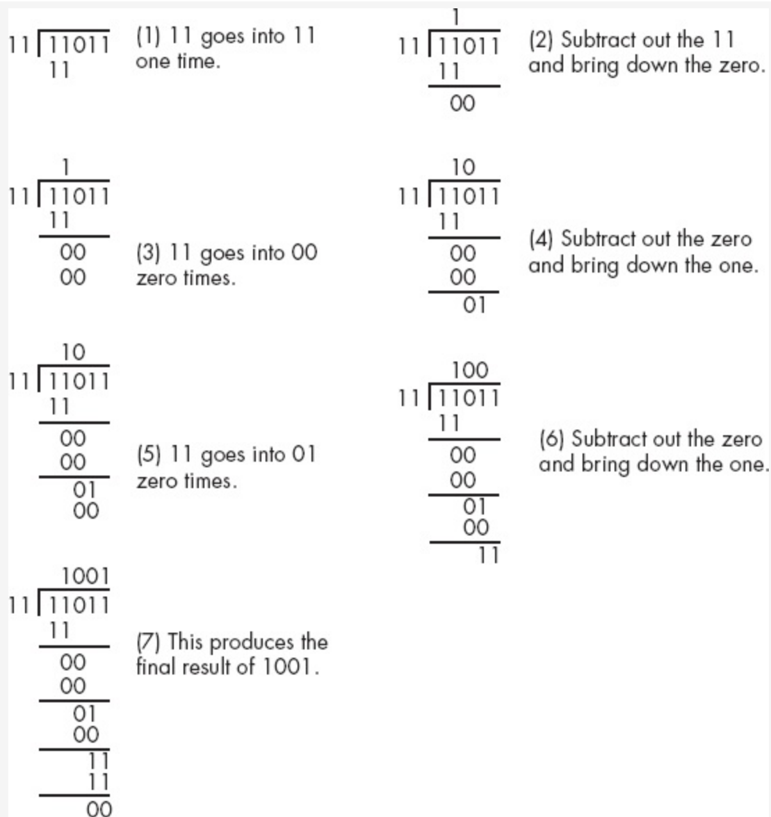
Figure 8-4. Longhand division in binary
