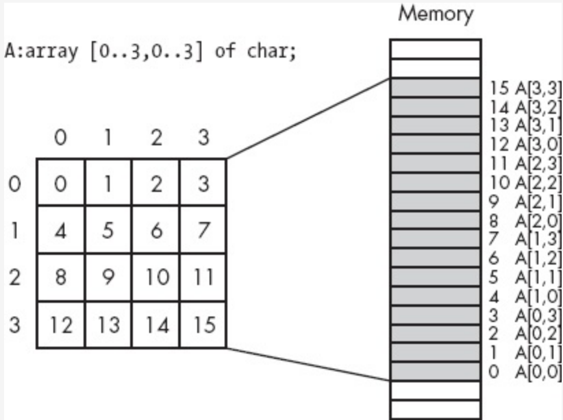
Figure 4-6. Row-major array element ordering
