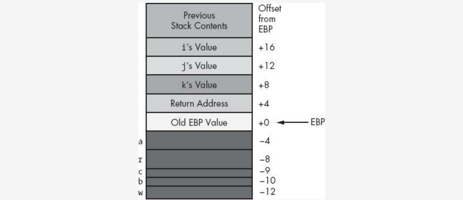
Figure 5-5. Offsets of objects in the ARDemo activation record
