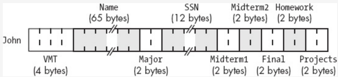
Figure 12-2. student class implementation in memory
