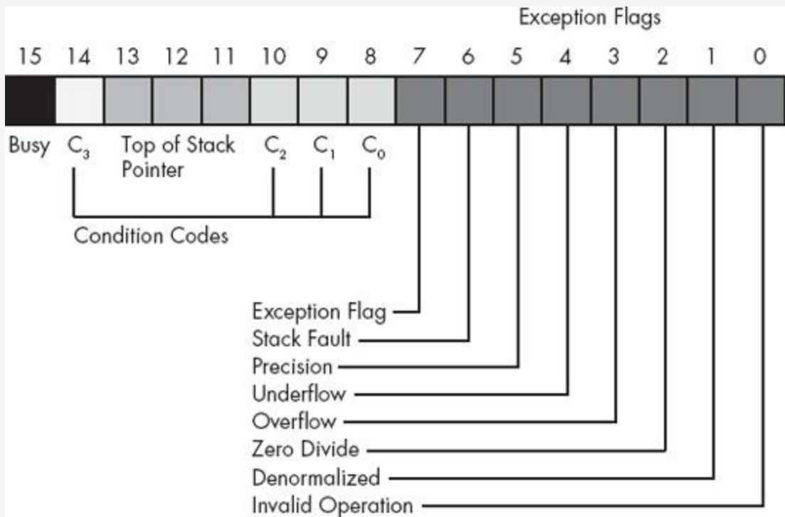
Figure 6-3. The FPU status register
