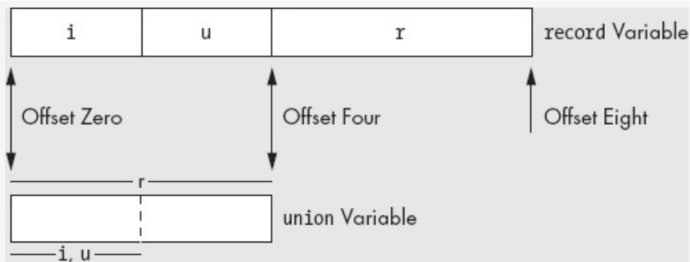
Figure 4-11. Layout of a union versus a record variable
