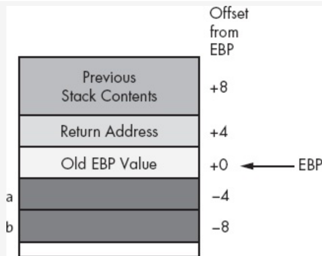
Figure 5-6. Activation record for the LocalVars procedure
