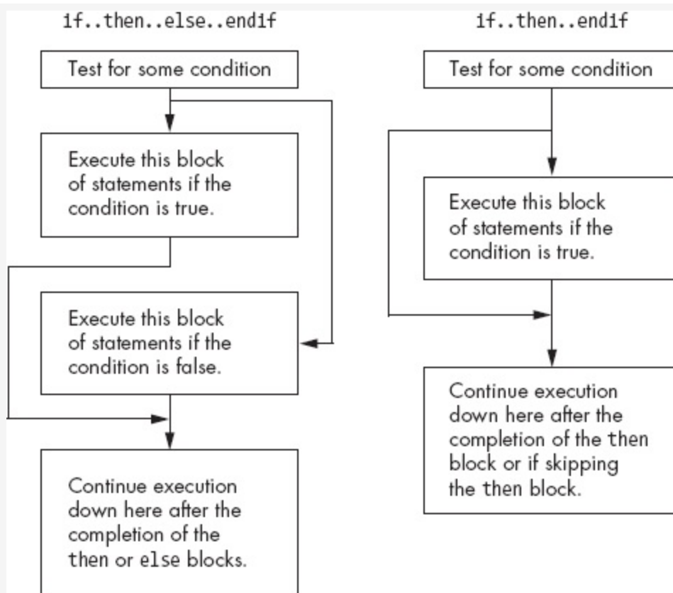
Figure 7-1. if..then..else..endif and if..then..endif statement flow
