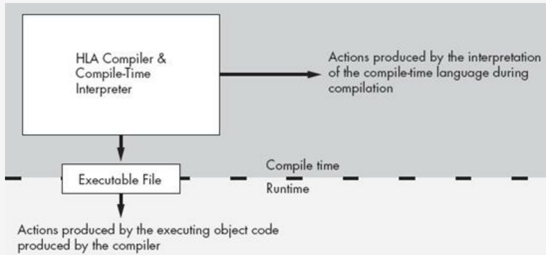
Figure 9-1. Compile-time versus runtime execution
