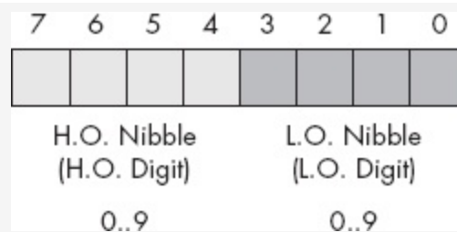
Figure 2-25. BCD data representation in memory
