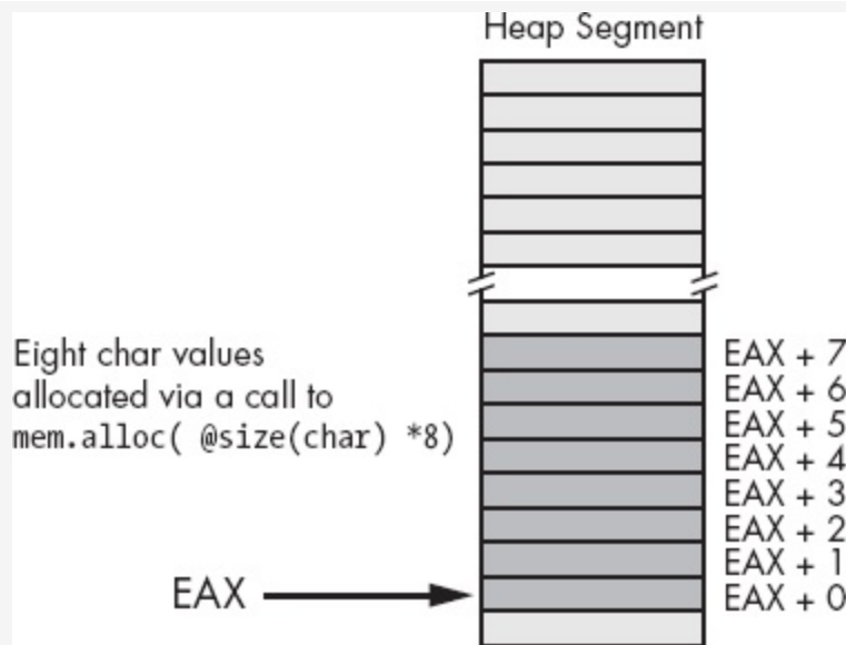
Figure 3-21. Allocating a sequence of eight character objects using mem.alloc
