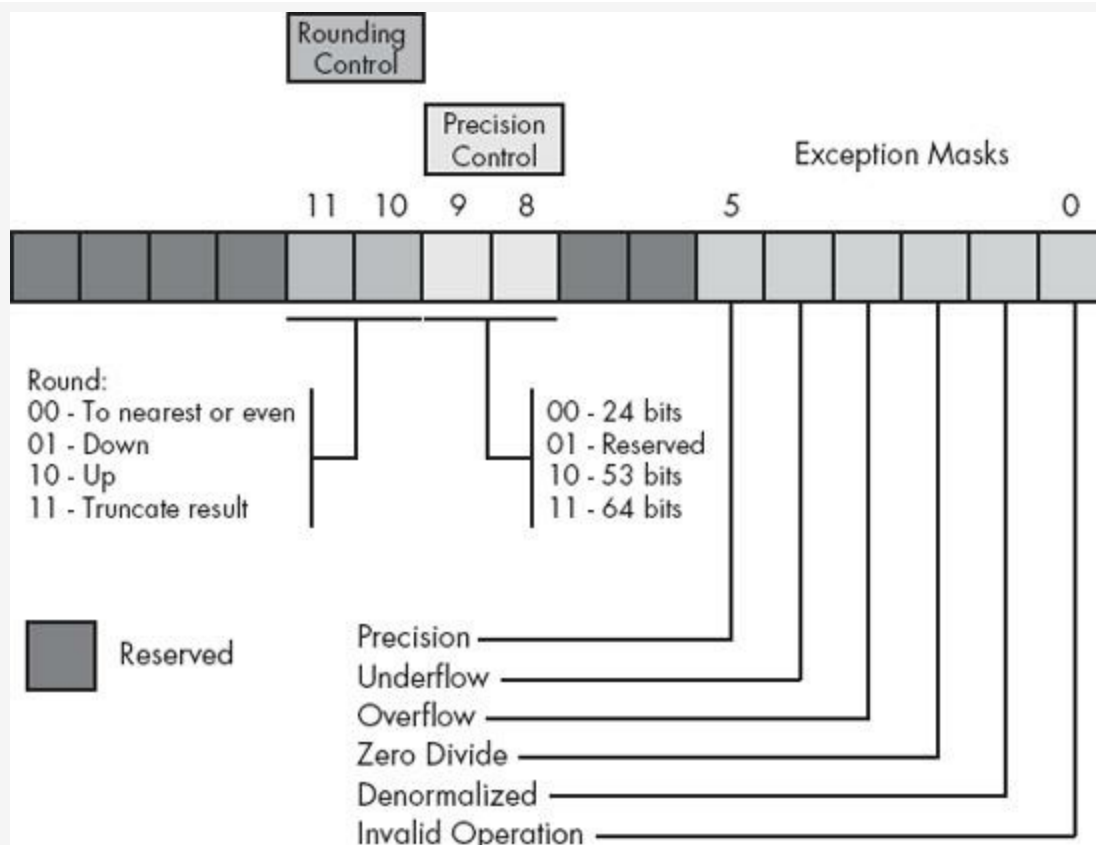
Figure 6-2. FPU control register
