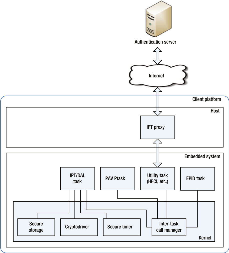
Figure 10-9. Architecture of the embedded IPT
