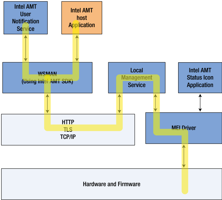
Figure 2-9. Local software components of the AMT
