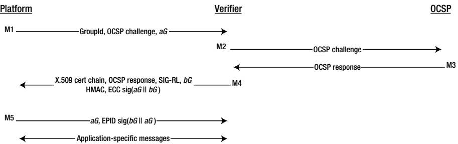
Figure 5-7. SIGMA protocol
