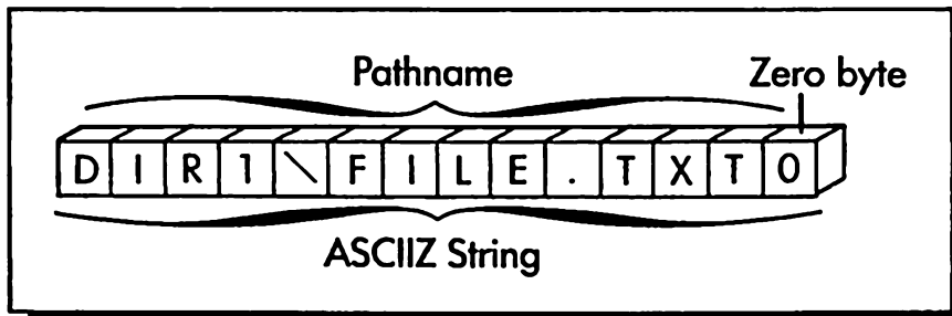
Figure 12-2. Pathname and ASCIIZ string
