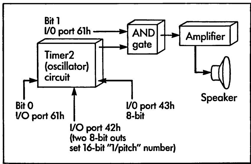
Figure 7-3. Sound hardware
