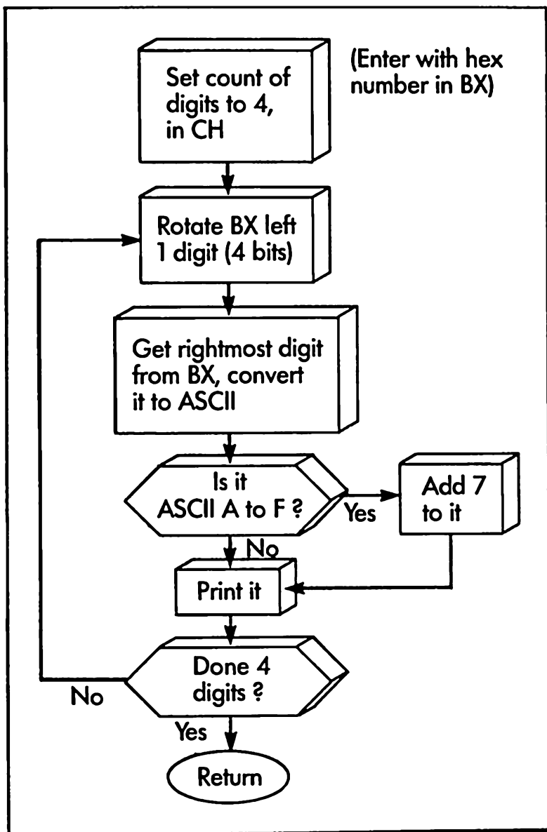
Figure 6-1. Flow chart of the BINIHEX program
