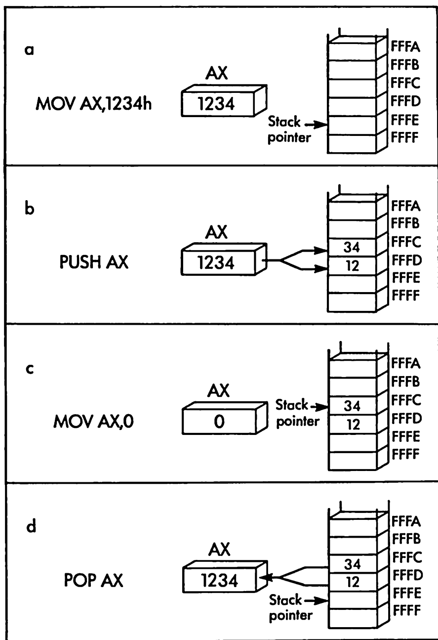
Figure 7-2. Operation of the stack
