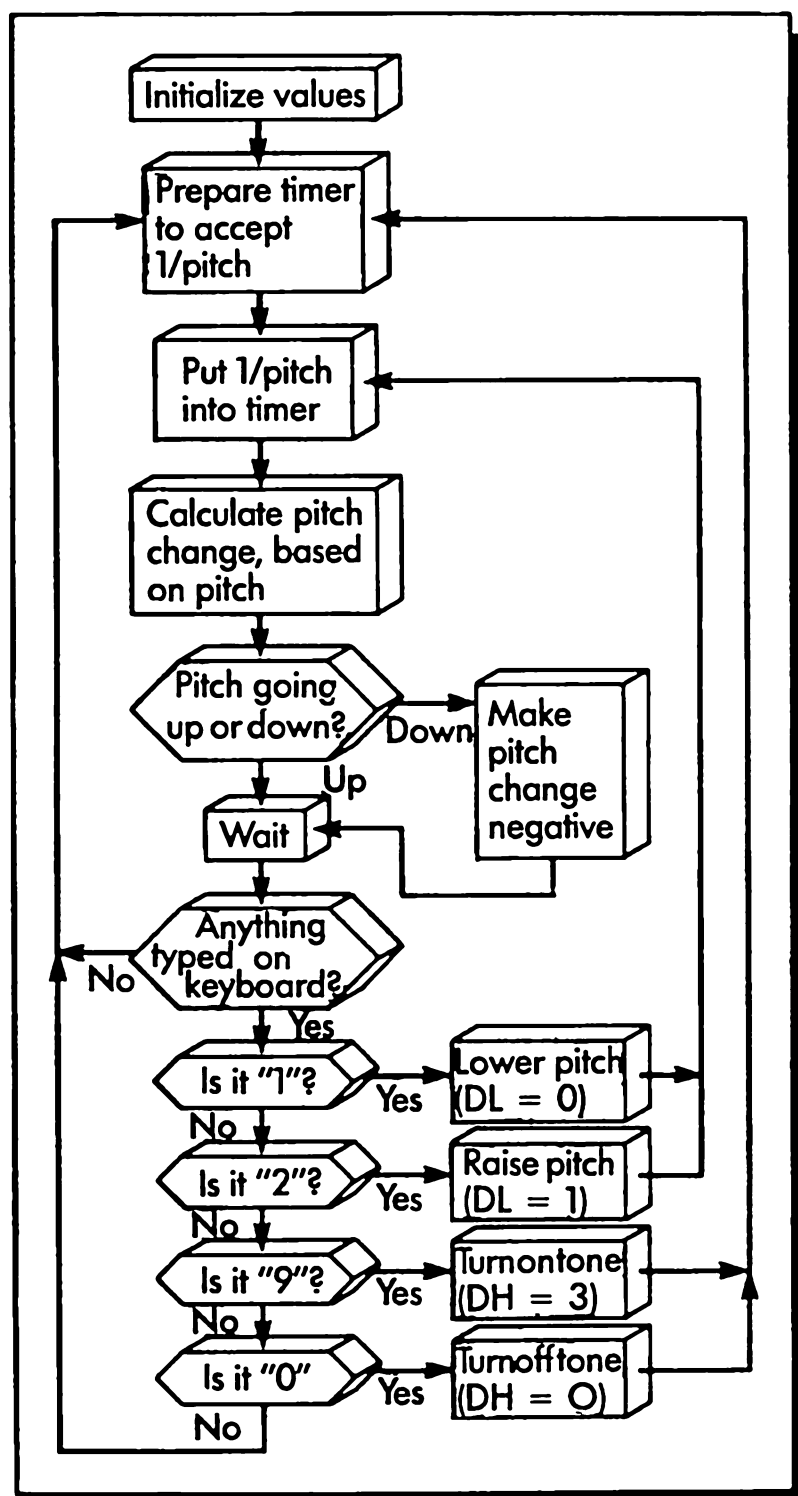
Figure 7-5. Flow chart of the KAZOO program
