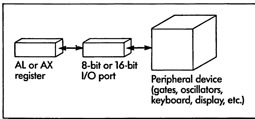
Figure 3-5. Input/output ports
