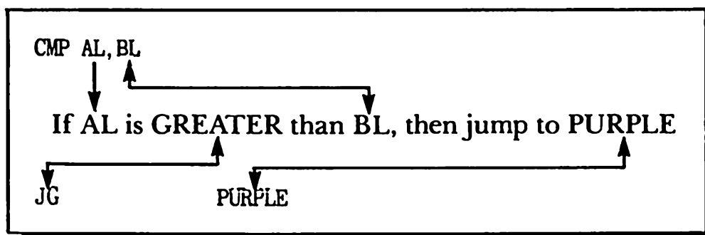
Figure 6-7. Comparisons and inequalities with JG
