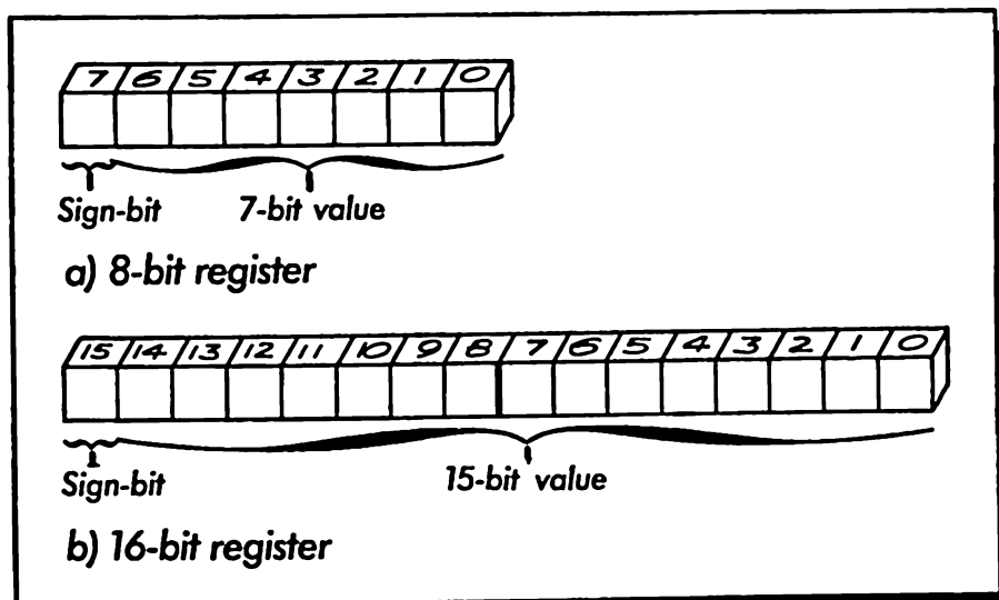
Figure 6-3. Signed numbers
