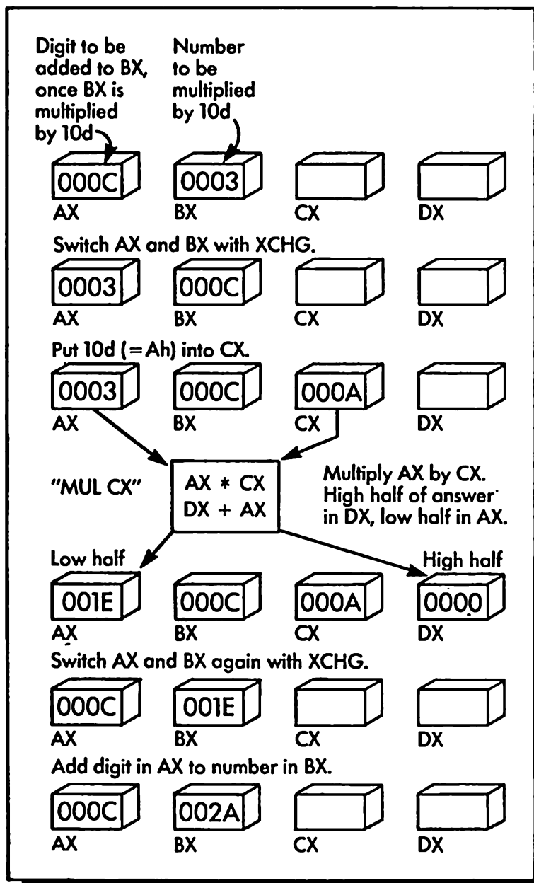
Figure 6-8. Operation of DECIBIN program
