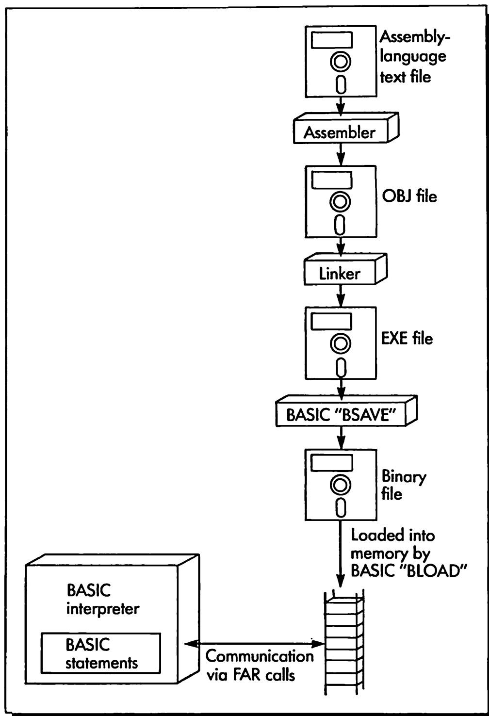
Figure 13-2. Assembly language and BASIC
