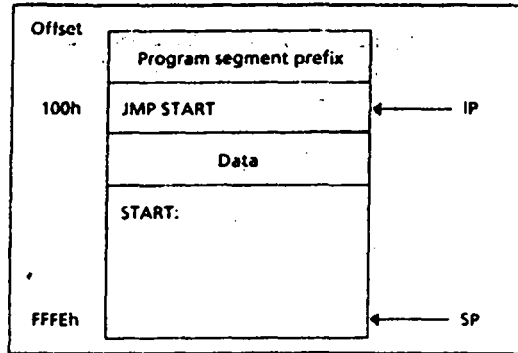
Figure 14.1 A .COM Program in Memory
