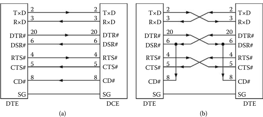
FIGURE 8.5 Equipment connection using the RS-232C interface. (a) Connection between a DTE and a DCE. (b) Null modem connection between two DTEs.
