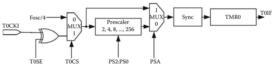
FIGURE 6.2 Block diagram for Timer0. Timer0 can count machine cycles (timer mode, T0CS = 0) or external pulses (counter mode, T0CS = 1). TMR0 is an 8-bit incrementing counter. When TMR0 overflows, it activates the flag T0IF in the INTCON register. Before reaching TMR0, the pulses are synchronized with the microcontroller’s clock. They might be affected by a programmable prescaler.
