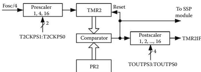
FIGURE 6.7 Timer2 block diagram.
