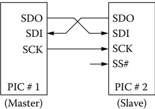
FIGURE 8.18 Two PIC microcontrollers connected using the SPI.
