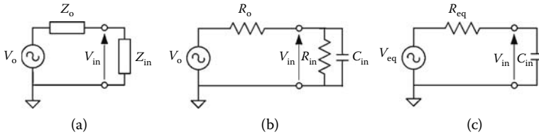
FIGURE 9.13 Equivalent circuits used to analyze voltage-loading effects for ac signals.
