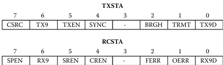
FIGURE 8.16 TXSTA and RCSTA registers used to control data transmission (TXSTA) and reception (RCSTA) in the USART serial port.
