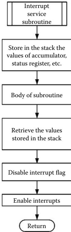
FIGURE 7.3 General structure of an interrupt service subroutine.
