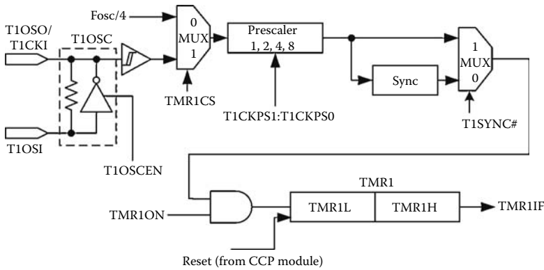
FIGURE 6.5 Timer1 block diagram.
