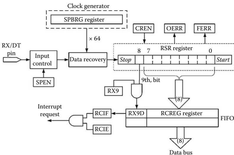
FIGURE 8.15 Receiver in the USART serial port.
