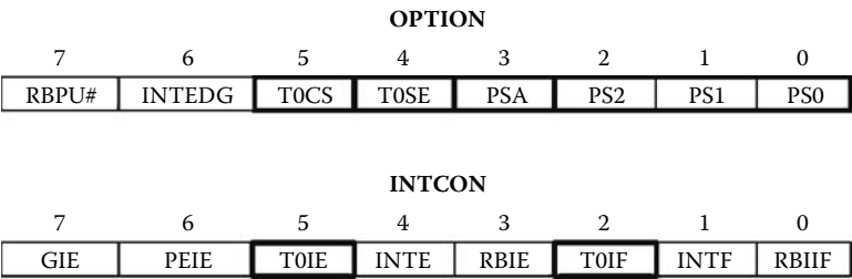
FIGURE 6.3 Special function registers OPTION and INTCON. OPTION stores the configuration bits for Timer0: T0CS configures Timer0 as a timer or counter; T0SE configures the external signal edge that will increment Timer0 when working as a counter; PSA assigns the prescaler to Timer0 or the watchdog; and PS2, PS1, and PS0 program the division factor for the prescaler. INTCON stores the Timer0 overflow flag, T0IF. Bit T0IE enables the interrupt request to the microcontroller as a result of Timer0 overflow.
