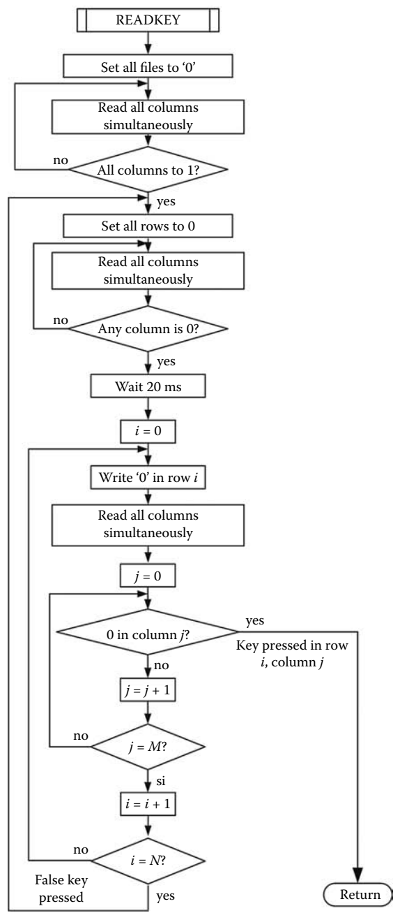
FIGURE 5.12 Algorithm to read an N -row, M -column matrix keypad using sequential exploration. The algorithm waits until a key is pressed and returns its position (row i , column j ).
