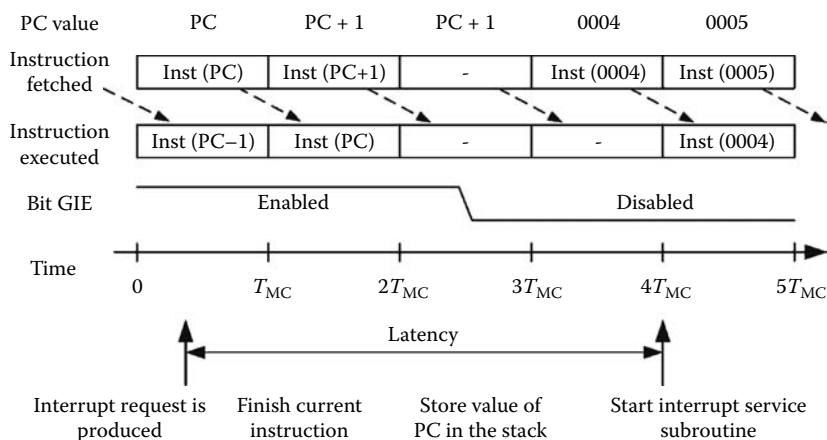
FIGURE 7.5 Microcontroller operations during latency time: the current instruction is finished, the value of the PC is stored in the stack, and the PC is loaded with 0004, causing it to execute the first instruction in the interrupt service subroutine. When this subroutine is executed, the interrupt system is disabled. The instruction retfie, used to return to the interrupted program, enables the interrupt system again.
