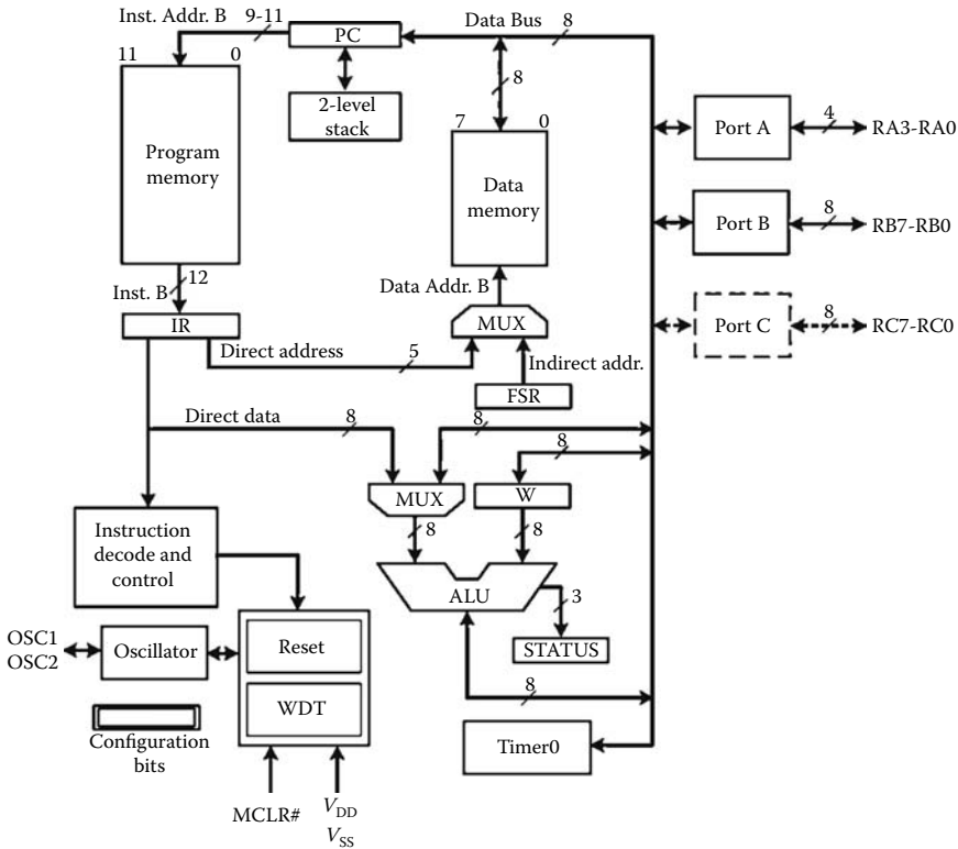
FIGURE 2.15 Internal architecture of PIC16X5xx family.
