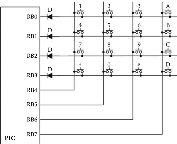
FIGURE 5.13 A 16-key matrix keypad connected to port B in a PIC. Diodes are used to avoid short circuits between two exploration lines if two or more keys in the same column are pressed simultaneously. This configuration uses the internal pull-up (not shown) available in port B to keep a logic 1 in the return lines when no keys are pressed.
