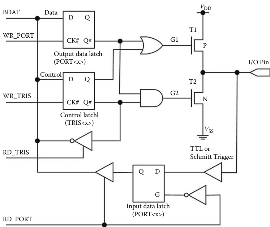
FIGURE 5.6 Basic schematic for a I/O pin in a medium-end PIC microcontroller.
