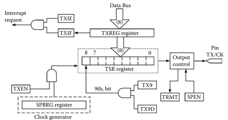
FIGURE 8.14 Transmitter in the USART serial port.
