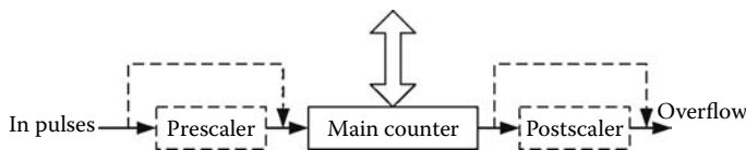
FIGURE 6.1 General block diagram for medium-end PIC timers. All of them have an 8-bit or 16-bit incrementing main counter and a prescaler. Timer2 also has a postscaler. The pulses to be counted can be internal or external. Overflow is reported in a bit from the special function registers. This bit can generate an interrupt request to the PIC.
