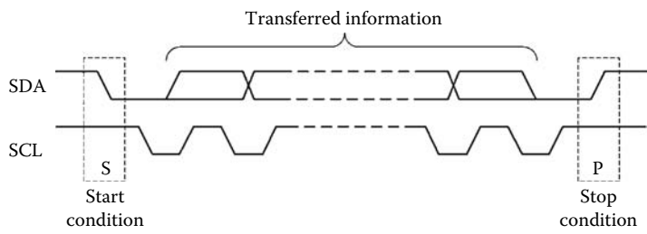
FIGURE 8.9 Start (S) and stop (P) conditions used by the master device to initialize and finish communication.
