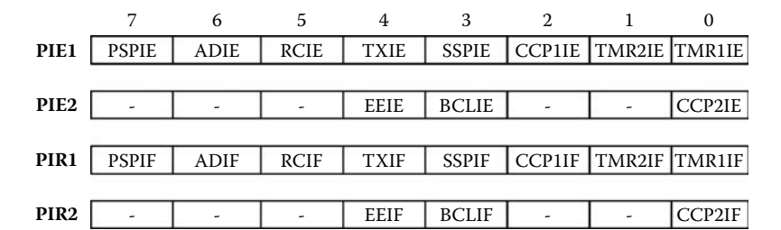
FIGURE 7.9 PIE and PIR registers in PIC16F87x microcontrollers.
