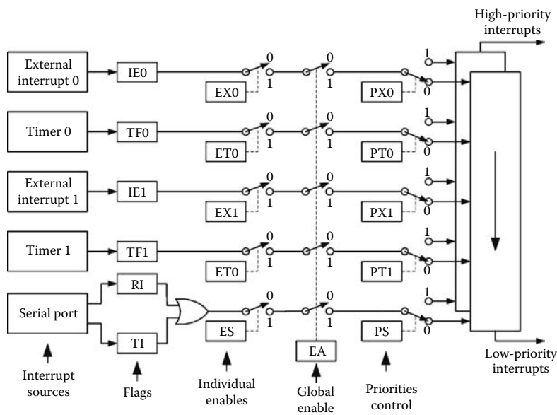
FIGURE 7.4 Interrupt system structure for a typical microcontroller in the MCS51 family.
