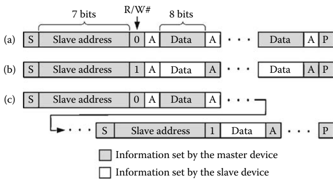
FIGURE 8.10 Communication format in three possible situations. (a) The master transmitter writes data in the slave receiver. (b) The master receiver receives data from the slave transmitter. (c) The master is initially a transmitter (R/W# = 0) and then becomes a master receiver, repeating the starting condition and sending the slave address by setting bit R/W# to 1.
