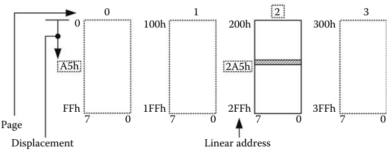
FIGURE 3.4 1 kB memory paged in 256 B pages showing the relationship between the linear address and the logical address. The linear address of the cell located in page 2 with a displacement A5h is 2A5h.
