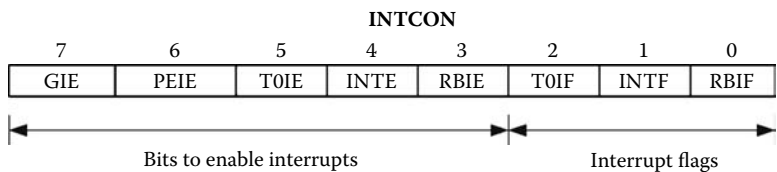
FIGURE 7.6 INTCON register for interrupt control.
