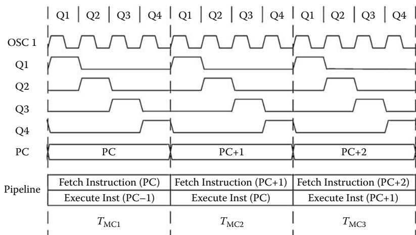
FIGURE 2.2 Clock signals in PIC microcontrollers. OSC1 is the main oscillator from which the internal signals Q1, Q2, Q3, and Q4 are derived. These signals synchronize fetching, decode, and execute of instructions. T_{MC} is the duration of a machine cycle. It uses four OSC1 pulses.
