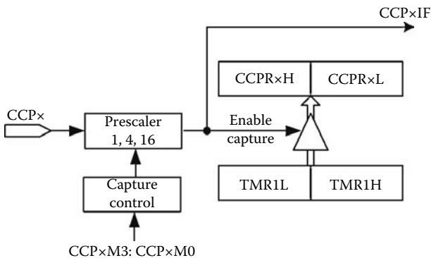
FIGURE 6.10 CCP module operating as a capture register for Timer1 for an event in pin CCPx.
