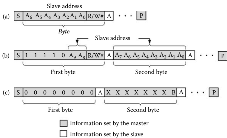
FIGURE 8.11 Addresses of devices connected to the I 2 C bus can be: (a) 7 bits or (b) 10 bits. (c) General call format.
