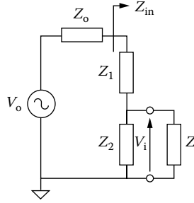
FIGURE 9.11 Voltage attenuator connected to a stage whose equivalent input impedance is Z_i .
