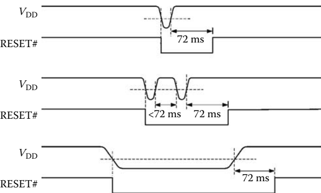
FIGURE 2.12 Reset signal due to brown-out in several situations. The timer PWRT guarantees that V_{DD} will be at its nominal value once it leaves the reset state.
