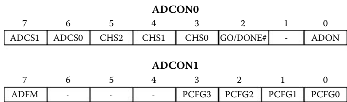
FIGURE 9.30 Registers ADCON0 and ADCON1 in a PIC16F873.
