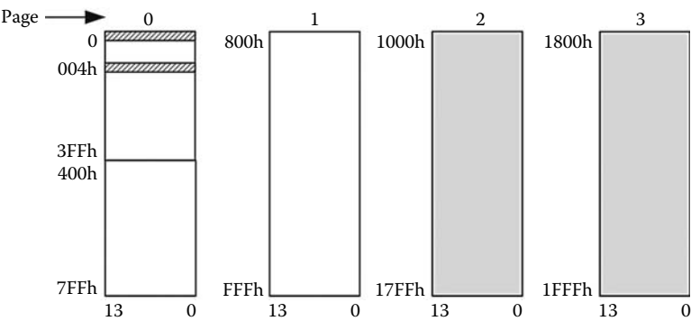
FIGURE 3.6 Program memory pages in medium-end PIC microcontrollers. They can have up to four pages of 2k words, each one with a total of up to 8k words. Each word is 14 bits long. The shadowed part is not part of the PIC16F873 because this microcontroller has 4k cells distributed between pages 0 and 1. The PIC16F84 only has the first 1024 memory cells that are located from address 0 to address 3FFh in page 0.
