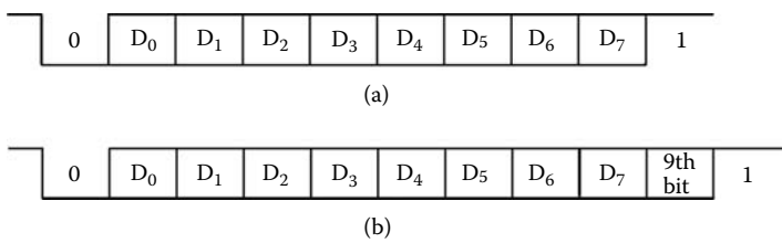
FIGURE 8.13 Format of the asynchronous signal in the serial port in medium-end PICs. (a) Data signal. (b) Data signal with the additional ninth bit.
