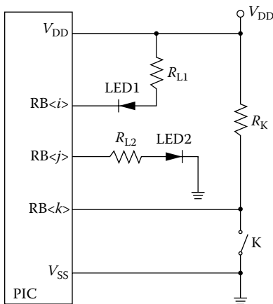
FIGURE 5.8 Connection of LEDs and switches to port B in a PIC microcontroller.
