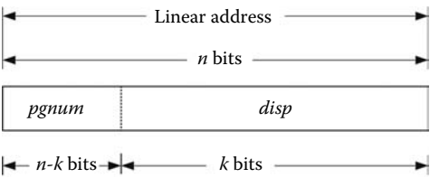
FIGURE 3.5 Linear address based on the components of logic address in a paged system when page size is a power of 2. The displacement ( disp ) takes the k least significant bits, and the page number ( pgnum ) takes the n - k most significant bits in the n bit linear address.
