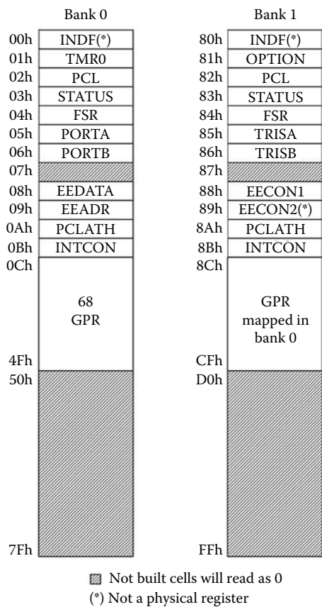
FIGURE 3.10 Data memory registers in the PIC16F84 microcontroller. These are organized in two banks with 68 general purpose registers (GPRs) that can be accessed from any bank, and 14 special function registers (SFRs). Some SFRs such as STATUS, PCLATH, PCL, FSR, and INTCON can be accessible from any bank. The first cell in each bank (INDF) is used for a data indirect address and it is not a real register in the microcontroller.
