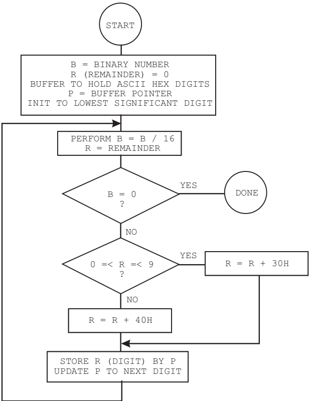
Figure 4-11 Unsigned Binary to ASCII Hexadecimal String
