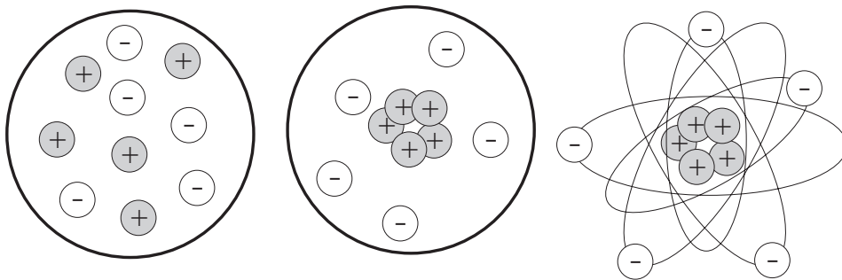
Figure 1-1 Models of the Atom
