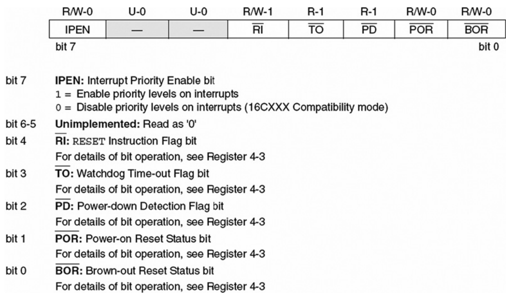
Figure 2.46: RCON register bits
