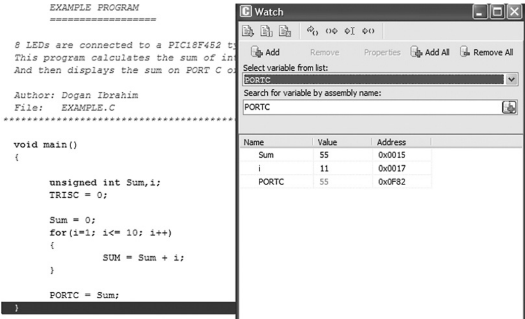
Figure 5.48: PORTC has the value 55
