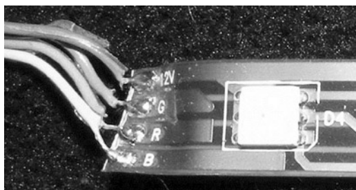
Figure 6-9. LED strip cut and wires soldered on
