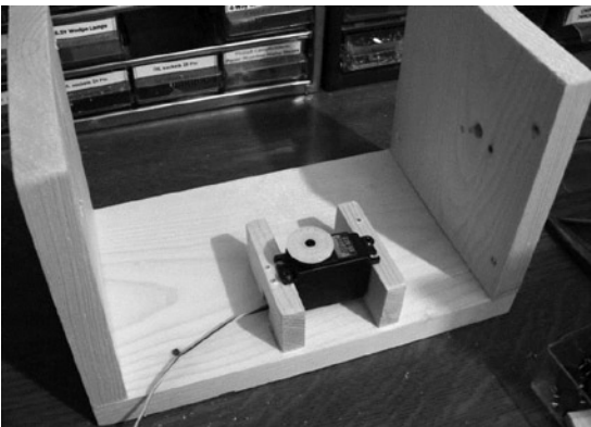
Figure 2-3. Crazy Beams project frame (vertical servo motor in place)
