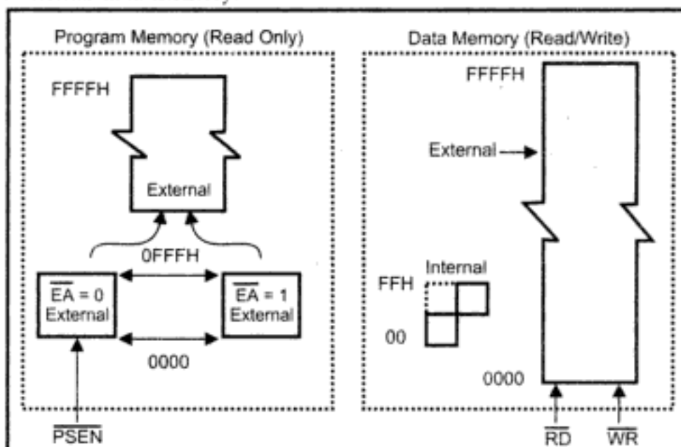
Fig. 11.8 Memory structure
