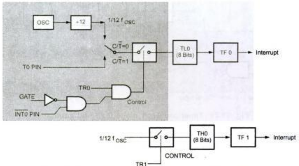
Fig. 11.23 Timer/counter 0 mode 3 : two 8-bit counters
