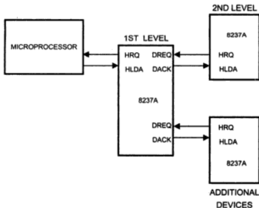
Fig. 6.14 Cascade 8237s
