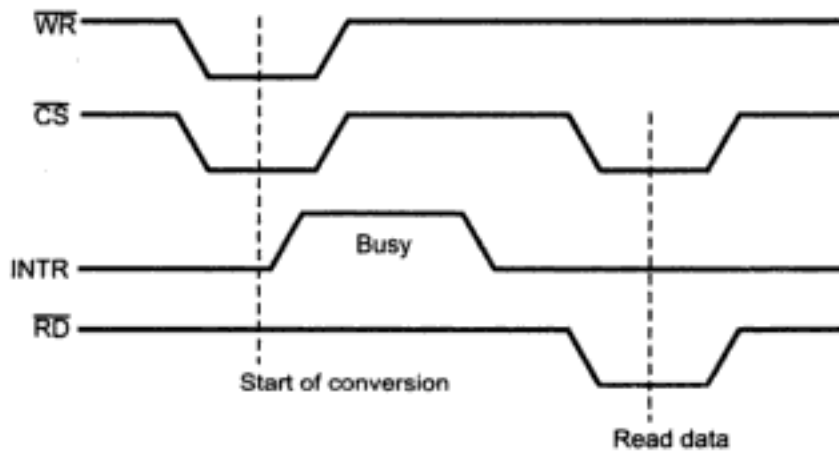
Fig. 7.34 Timing diagram
