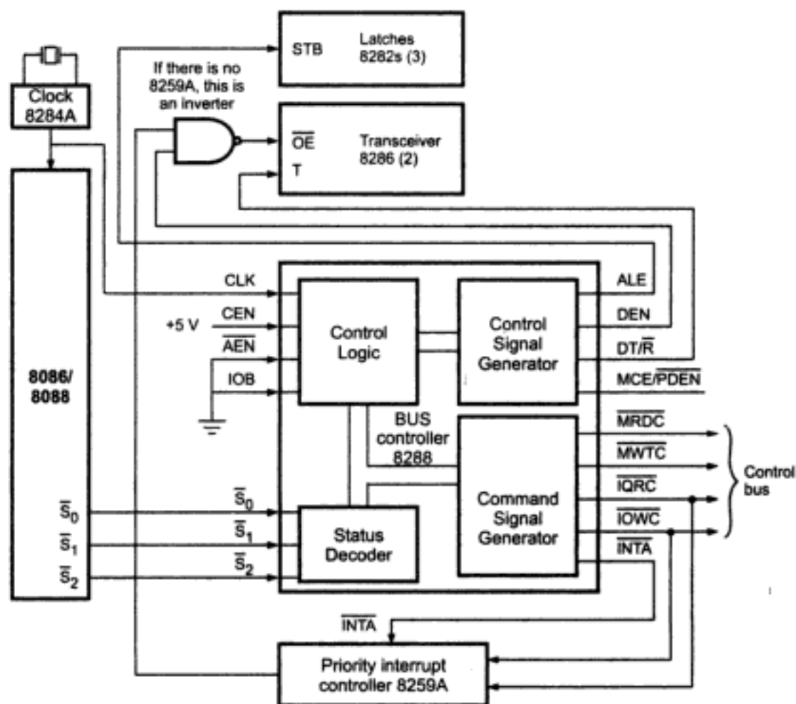
Fig. 5.16 8288 bus controller
