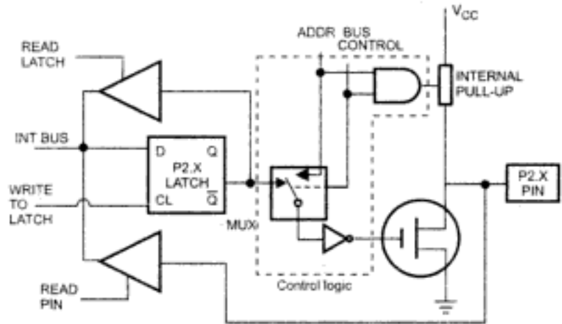
Fig. 11.9 (c) Port 2 bit
