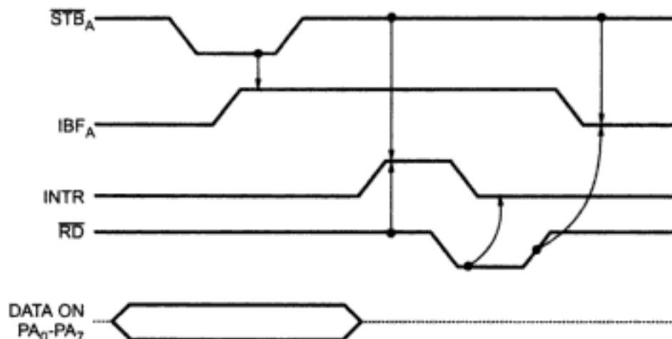
Fig. 7.8 (b) Timing diagram for port A in mode 1
