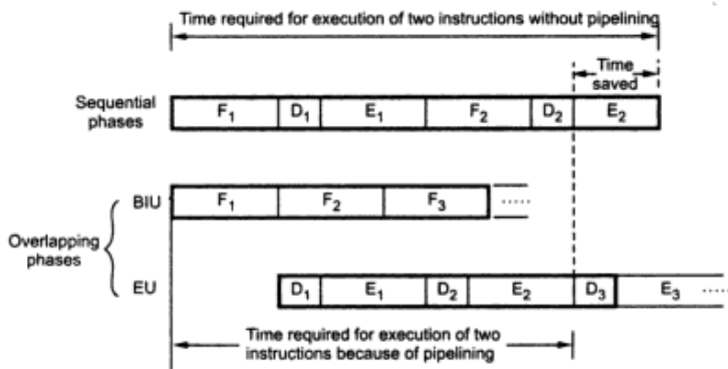
Fig. 2.3 Pipelining
