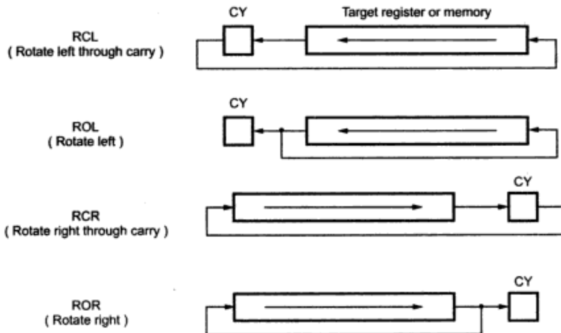
Fig. 3.19 Rotate operations
