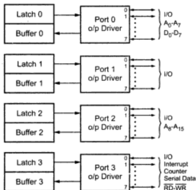
Fig. 11.4 I/O Ports
