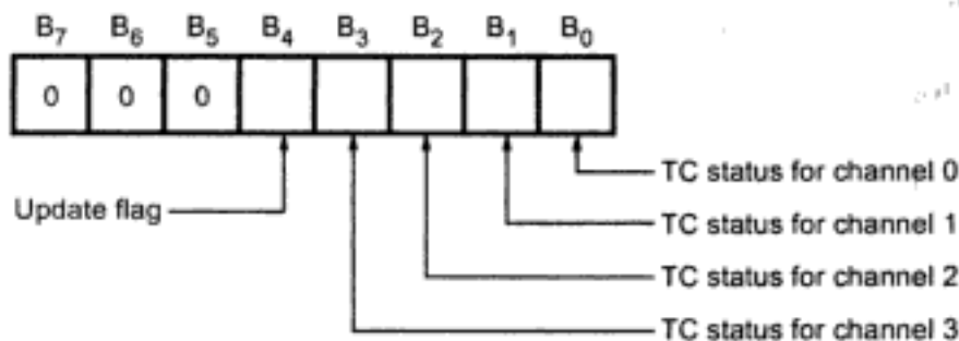
Fig. 6.8 Status register
