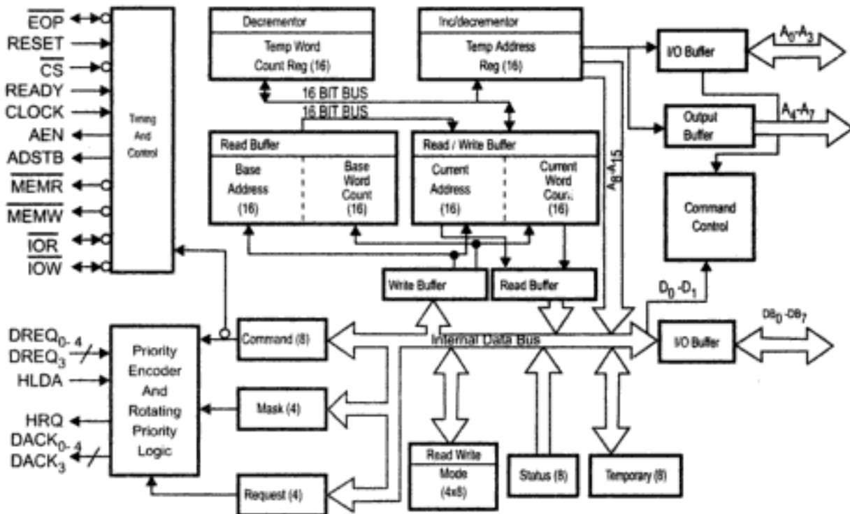
Fig. 6.12 Internal block diagram of 8237A
