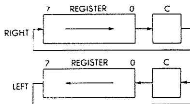
Fig. 4.11: Nine-Bit Rotation
