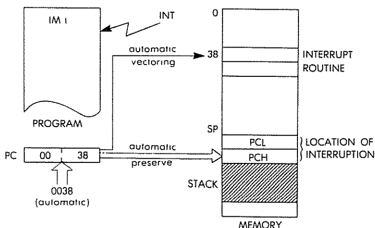
Fig. 6.28: Mode 1 Interrupt
