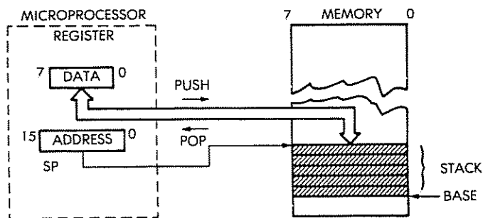
Fig. 2.5: The Two-Stack Manipulation Instructions
