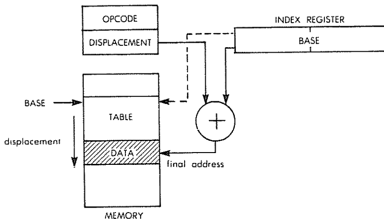
Fig. 5.2: Addressing (Pre-indexing)
