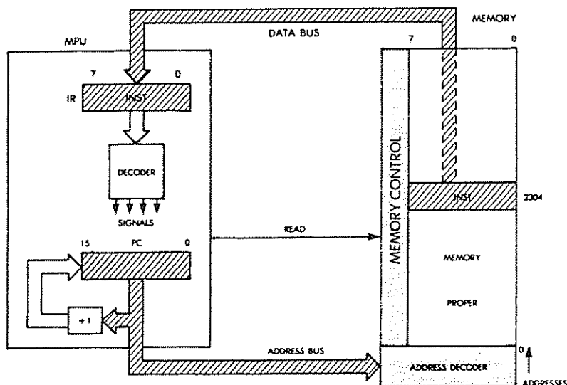
Fig. 2.7: Automatic Sequencing
