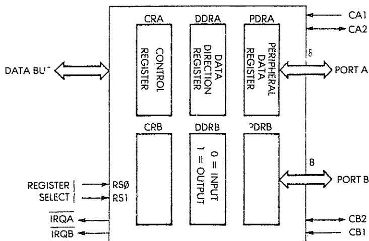
Fig. 7.1: Typical PIO
