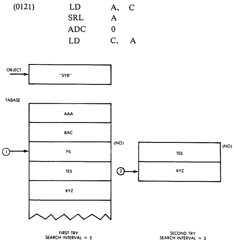
Fig. 9.19: A Binary Search
