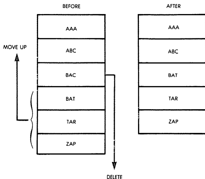
Fig. 9.21: Delete "BAC"
