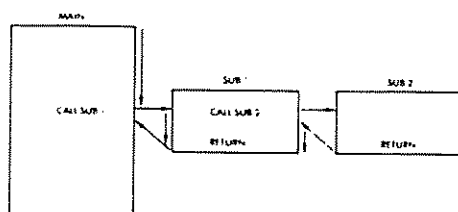
Fig. 3.36: Nested Calls
