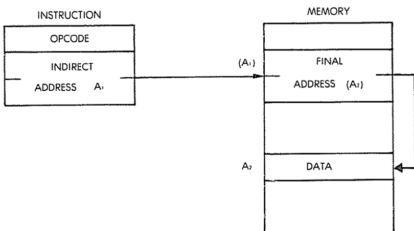
Fig. 5.4: Indirect Addressing
