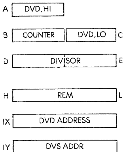
Fig. 3.34: Non-Restoring Division—The Registers
