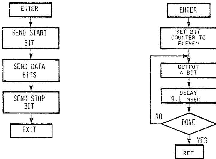
Fig. 6.16: Teletype Output
