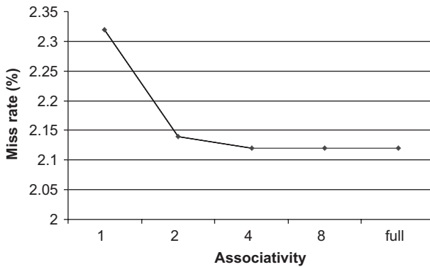
Figure 2.17. Miss rate vs. associativity. The data cache is (32\text{ KB},m,64) with the associativity m ranging from direct-mapped (1) to full. The application and the source are the same as in Figure 2.16.
