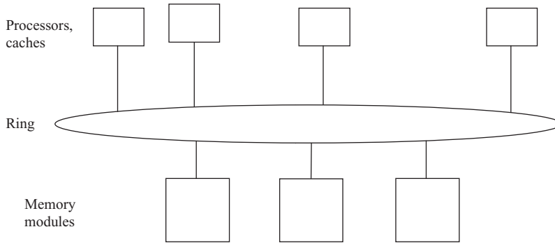
Figure 7.5. Ring interconnect.
